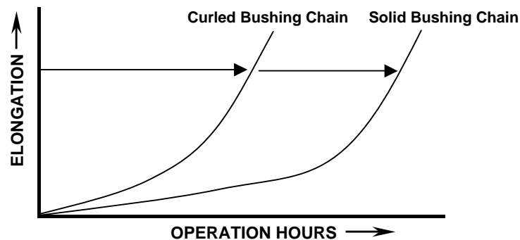
■ WEAR RESISTANCE CHART
